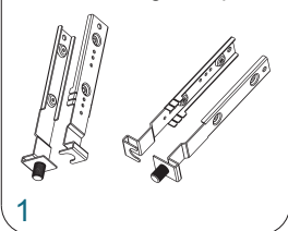
Assembled T-grid Clips, x2
