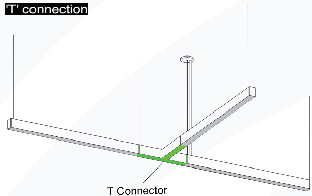
'T' connection
