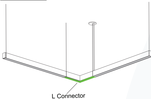
'L' connection
