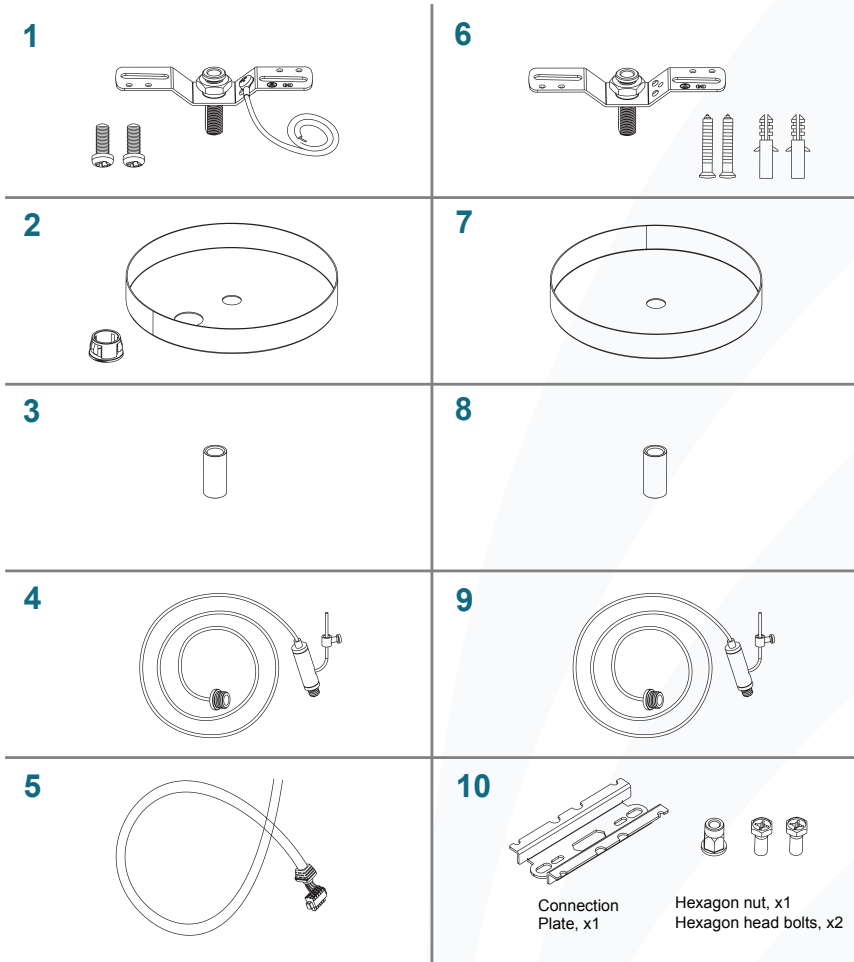
Power-Feed Suspension Kit
